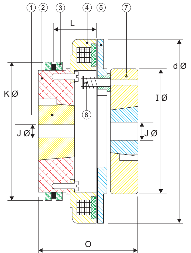
CLUTCH WITH SLIPRING, ARMTURE PLATE WITH TAPER LOCK
