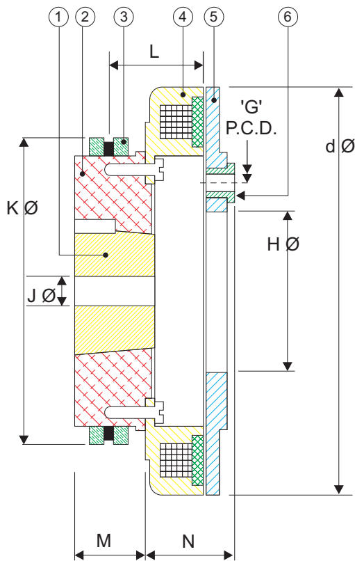
CLUTCH WITH SLIPRING, ARMTURE PLATE WITHOUT TAPER LOCK
