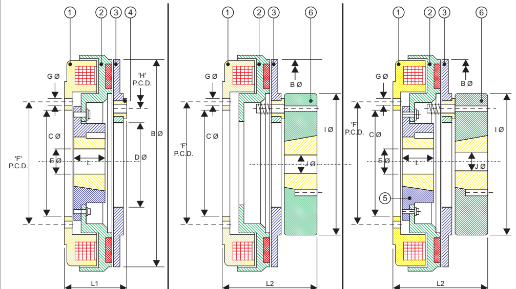
INTERNAL MOUNTING CLUTCH TAPER LOCK AT ROTOR SIDE
