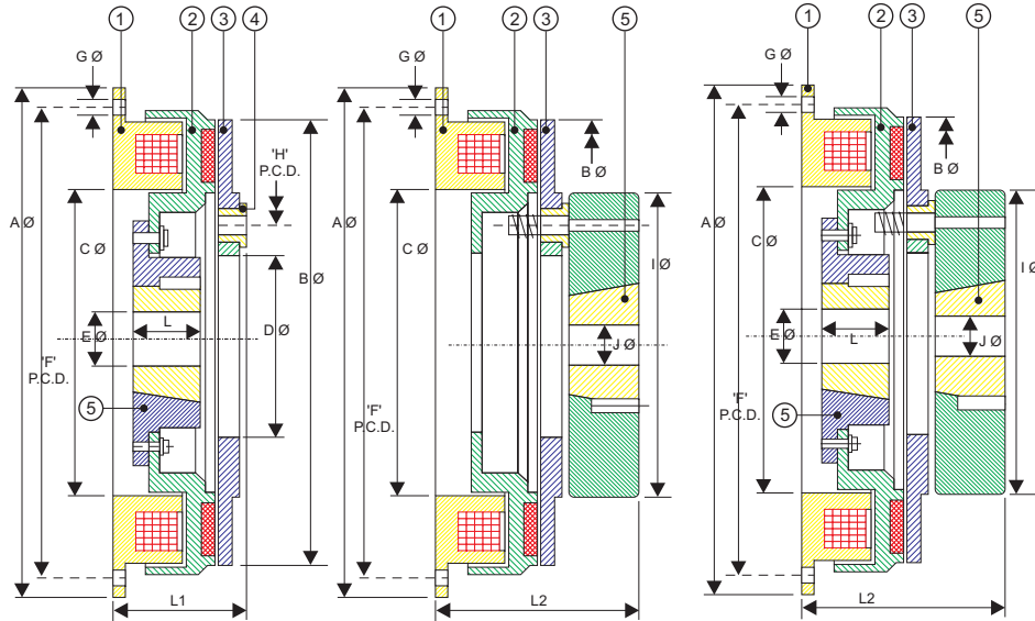
EXTERNAL MOUNTING CLUTCH TAPER LOCK AT ROTOR SIDE
